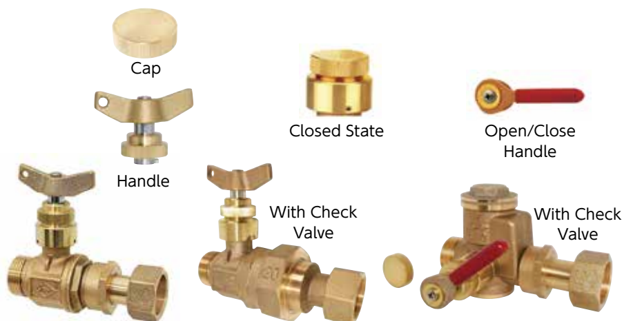
NT-M Retractable Ball Valve NT-M-MEO 13~25
